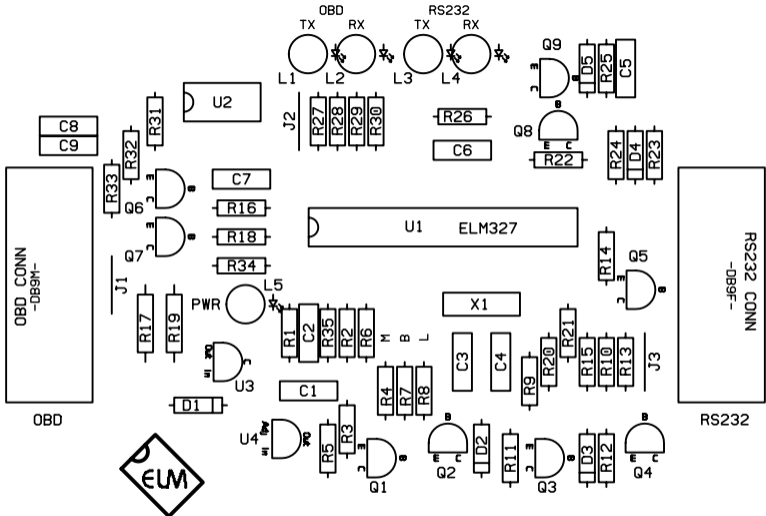
ELM327 DEMO BOARD
